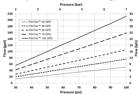
Figure 1: Impact of Pressure on Target Permeate Flow
