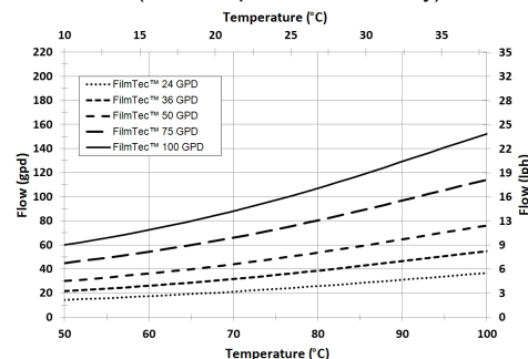
Figure 2: Impact of Temperature on Target Permeate Flow
